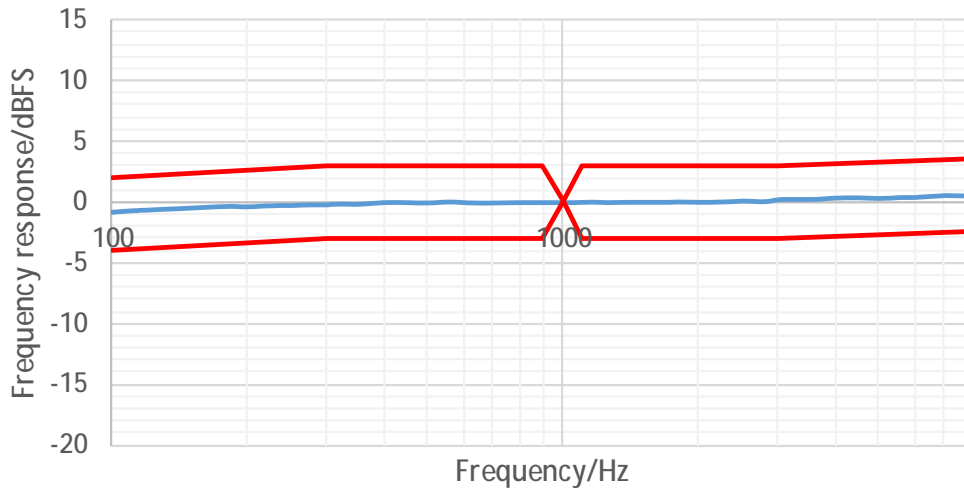
Typical Free Field Response Normalized to 1kHz Low Power Mode V_{DD}=1.8V , f_{CLK}=768kHz , Decimation Rate=48x
